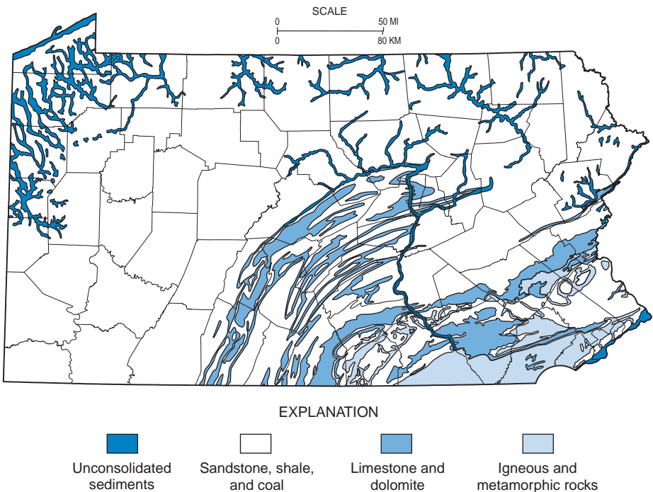
Distribution of rocks and sediments in Pennsylvania.
