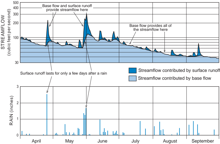
Relationship between streamflow and precipitation near Allentown, Pa., in 1968.
