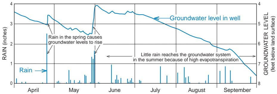
Relationship between groundwater level, precipitation, and season near Allentown, Pa., in 1968.
