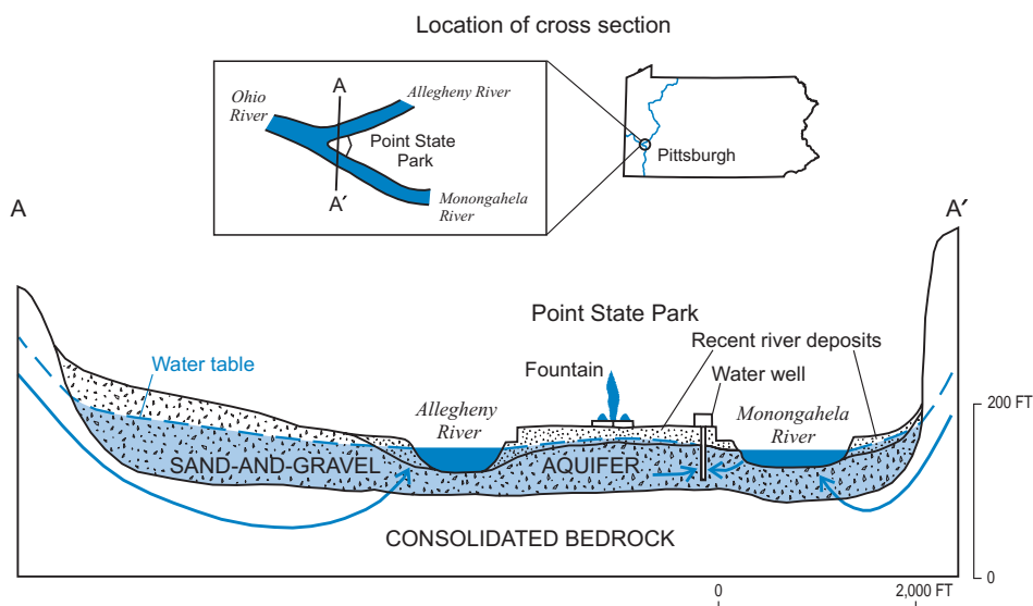
Cross section of the Allegheny and Monongahela River valleys at Point State Park, Pittsburgh. The vertical scale is greatly exaggerated to show detail.
