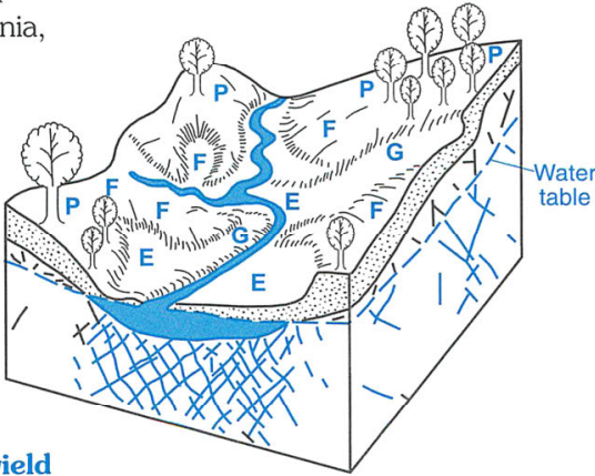
How topography reflects well-yield potential: E, excellent; G, good; F, fair; and P, poor.
