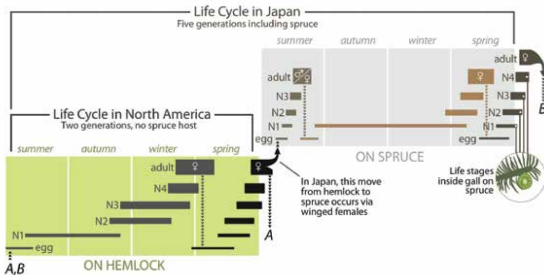
Figure 5. Multi-generation life cycle of HWA in its native range in Japan and its introduced range in eastern North America (Diagram: Vince D’Amico and Nathan Havill, USDA Forest Service.)
