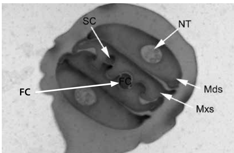
Figure 11. Cross-section of hemlock woolly adelgid stylets. FC, food canal; Mds, mandibular stylet; Mxs, maxillary stylet; NT, neurotubules of mandibles; SC, salivary canal. Scale bar= 1 \mu m (Photo: Kelly Oten, NC State University).
