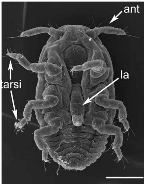
Figure 9. Ventral view of an HWA crawler. Scale bar = 100 \mu m. ant, antenna; la, labium (Photo: Kelly Oten, NC State University).
