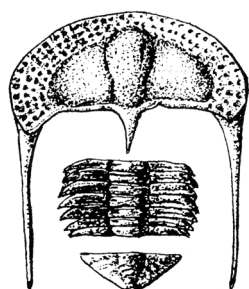
Figure 19. The trilobite genus Cryptolithus . A. Sketch of a specimen showing the cephalon (head), thorax (body), and pygidium (x4). B. Side view of the cephalon showing the free cheeks, which have rearward-pointing spines (x4).
