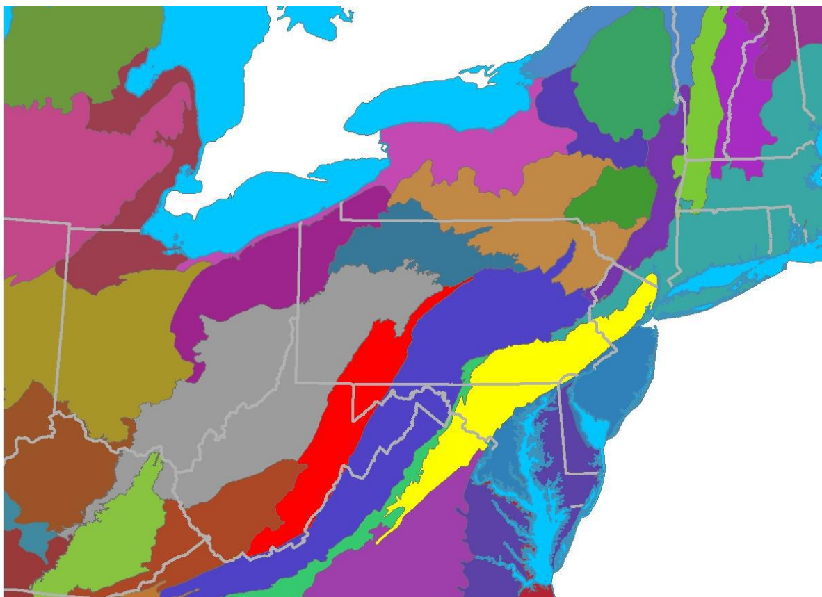
Figure 1. Ecomap Ecological Regions (USDA Forest Service, 1993). The Bureau considers a species native if it was present in Pennsylvania at the time of European colonization or if it naturally occurs within one of the zones that extends into Pennsylvania, as shown on this map.
